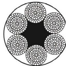
6X111SWSNS+FC
