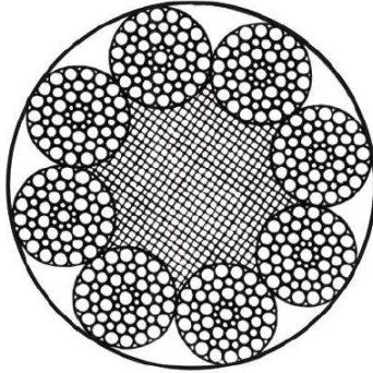
8x55SWS+FC
