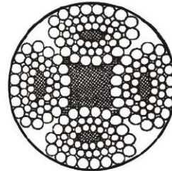
4Vx48S+5FC
