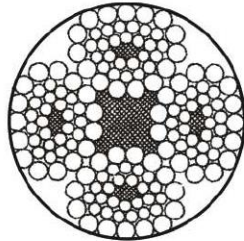
4Vx39S+5FC
