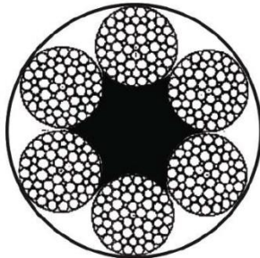
6x61FWS+FC
