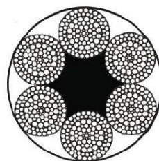
8X109SWSNS+FC
