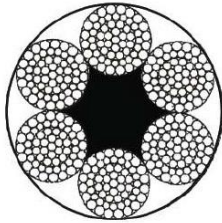
6X65FNS+FC
