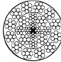
24Wx7
