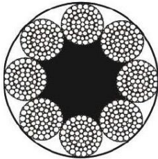
8X65FNS+FC
