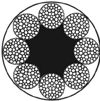
8x61FWS+FC
