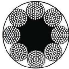
8x61+FC
