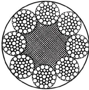
8X36WS+FC
