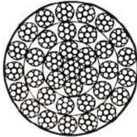
34x7+IWS
