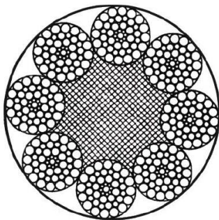
8x49SWS+FC
