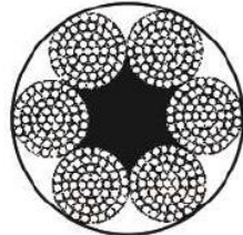
6x61+FC
