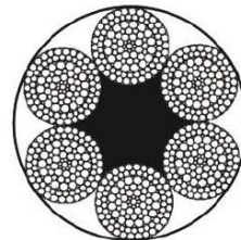
6X109SWSNS+FC
