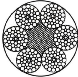
6x49SWS+FC
