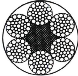
6x36WS+FC
