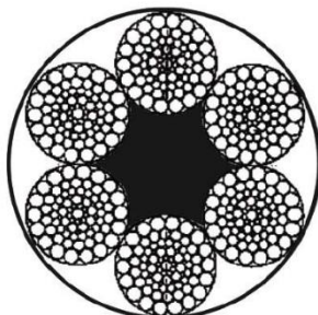
6x64SFS+FC
