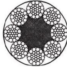
8x31WS+FC
