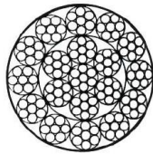
18x7+IWS
