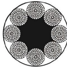
8X111SWSNS+FC
