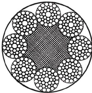
8x41WS+FC
