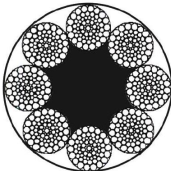
8x64SFS+FC
